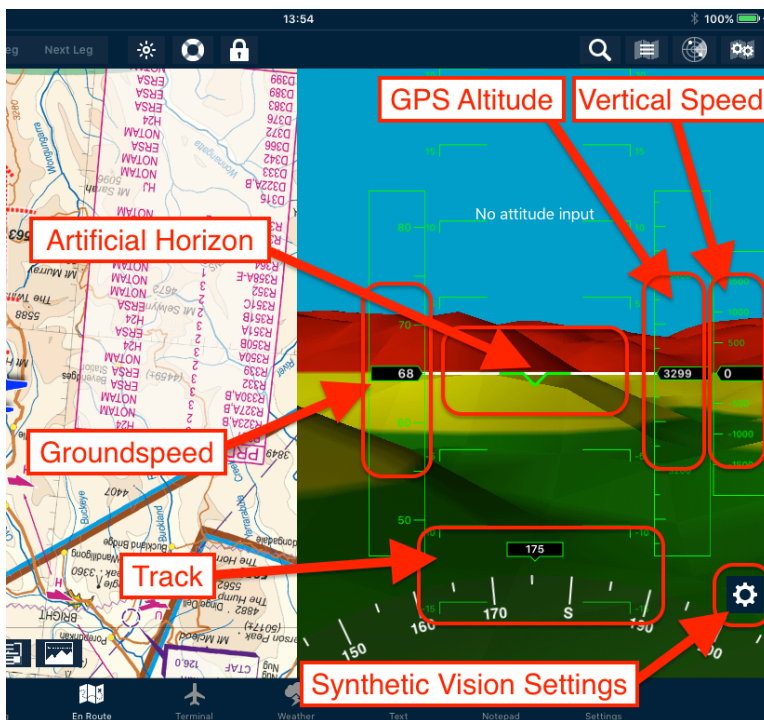
Figure 45 - Synthetic Vision layout
