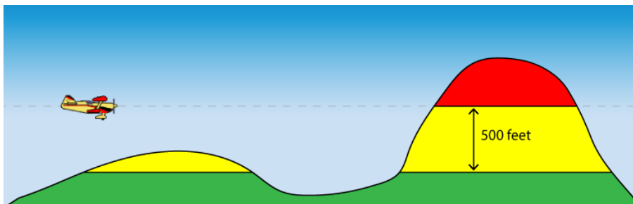
Figure 46 - Terrain Shading
